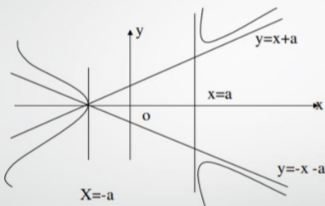
Graph of y^2(x-a) = x^2(x+a)
